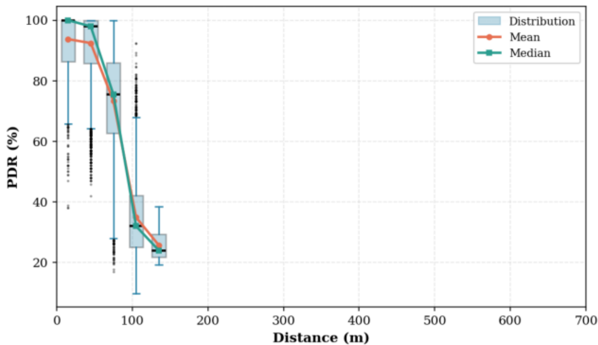
8_ECDSA_D_NLOS [ECDSA P-256]
