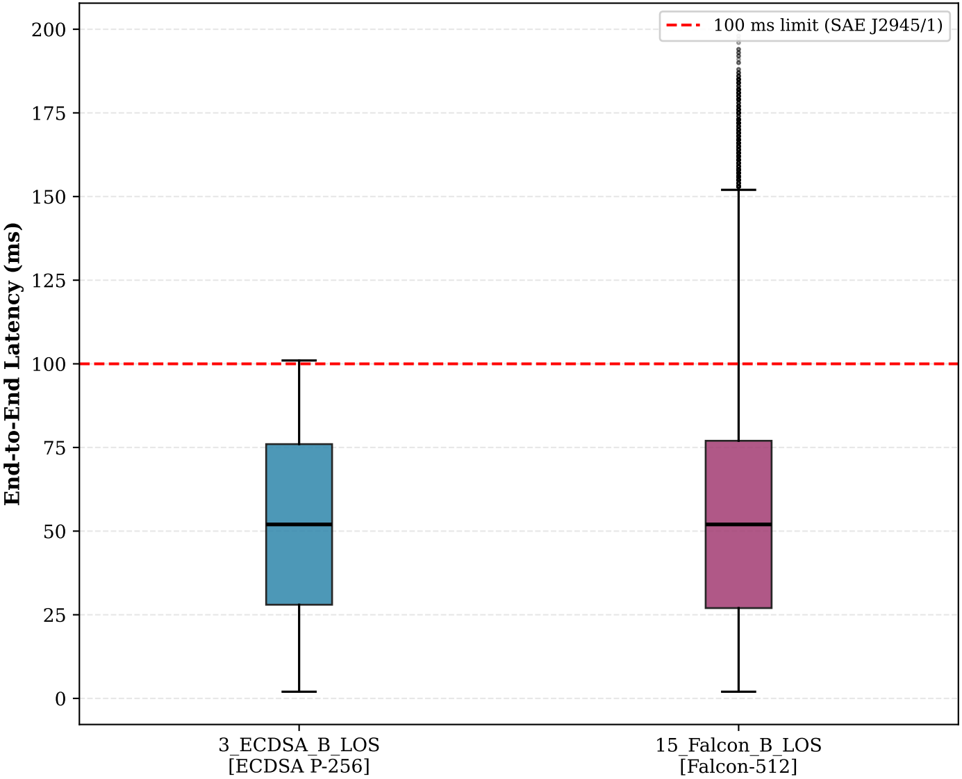
Latency Comparison — Scenario 3 vs Scenario 15
