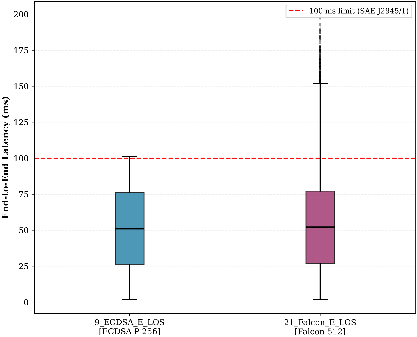
Latency Comparison — Scenario 9 vs Scenario 21
