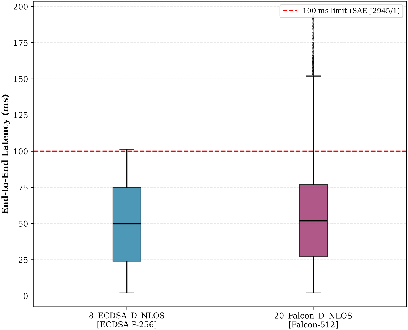
Latency Comparison — Scenario 8 vs Scenario 20
