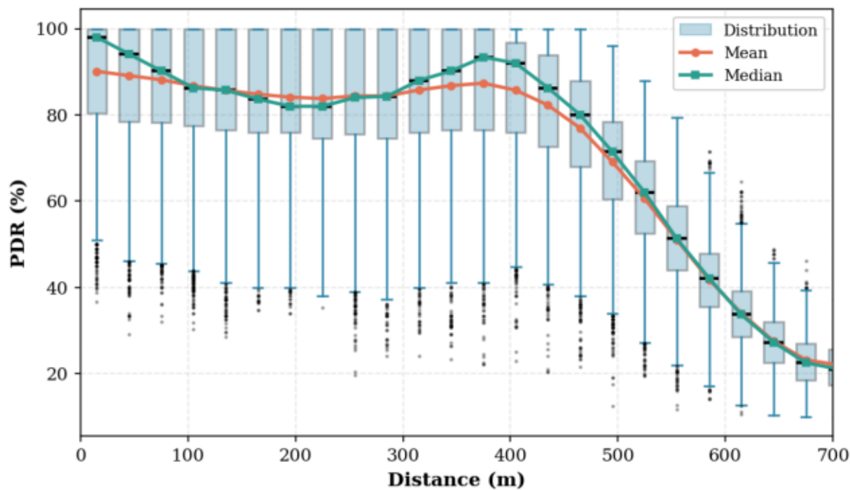
9_ECDSA_E_LOS [ECDSA P-256]
