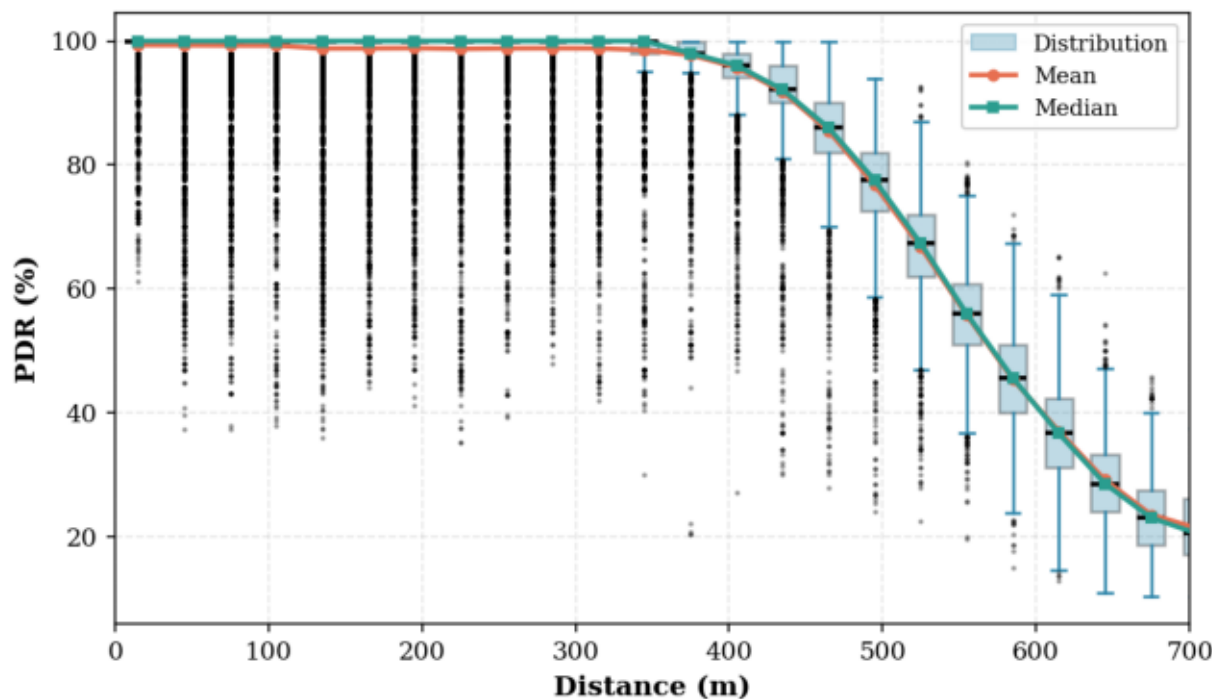
5_ECDSA_C_LOS [ECDSA P-256]
