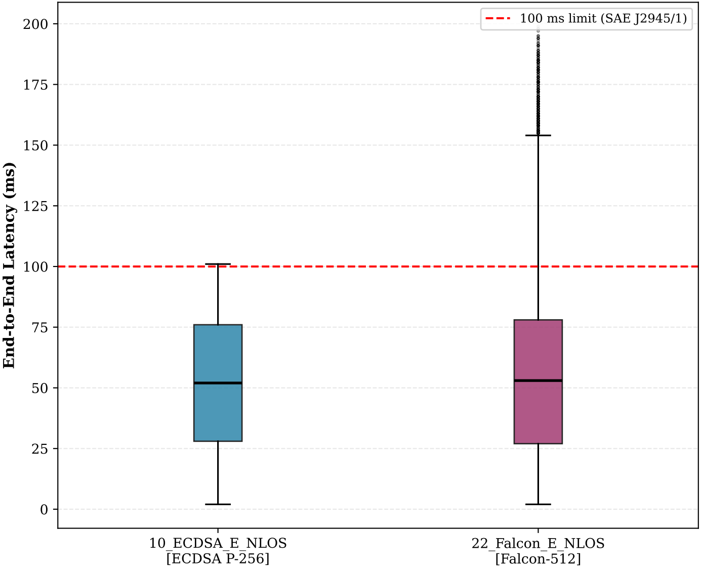
Latency Comparison — Scenario 10 vs Scenario 22
