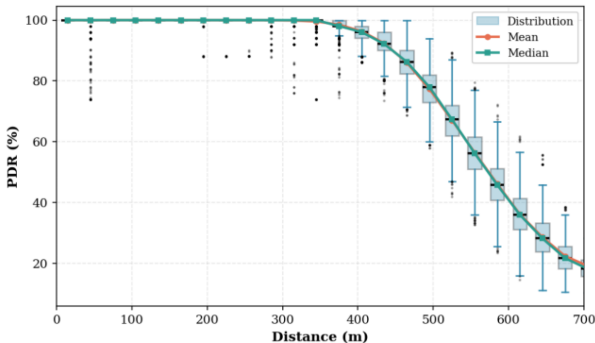
1_ECDSA_A_LOS [ECDSA P-256]
