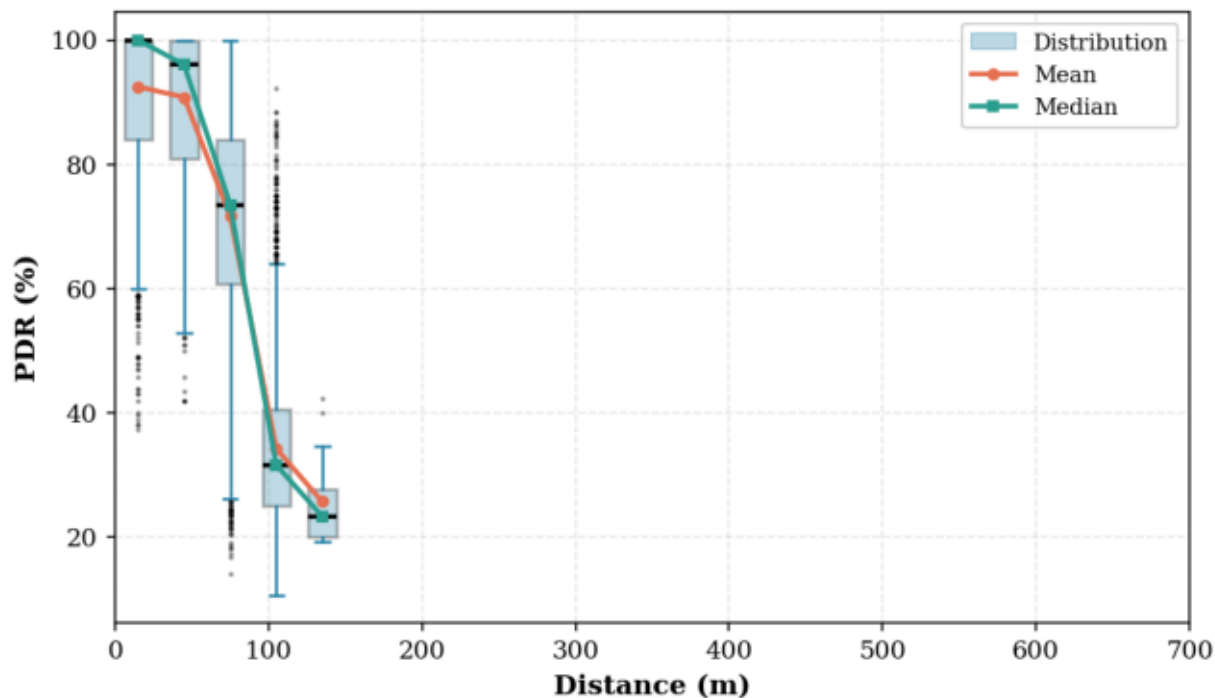
10_ECDSA_E_NLOS [ECDSA P-256]
