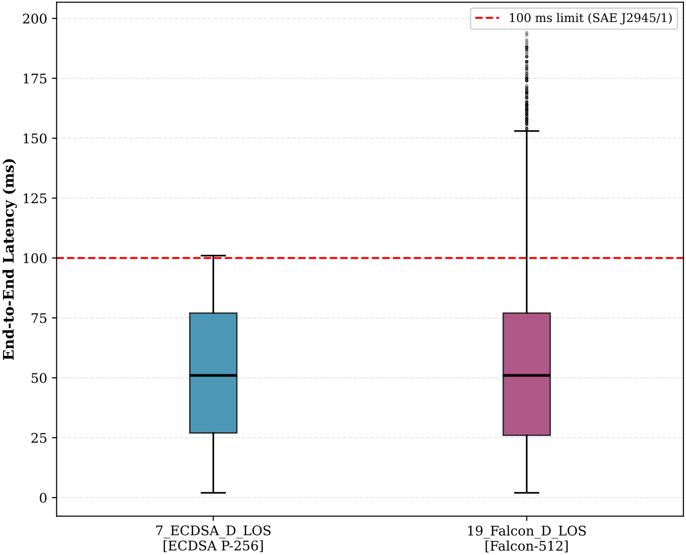
Latency Comparison — Scenario 7 vs Scenario 19
