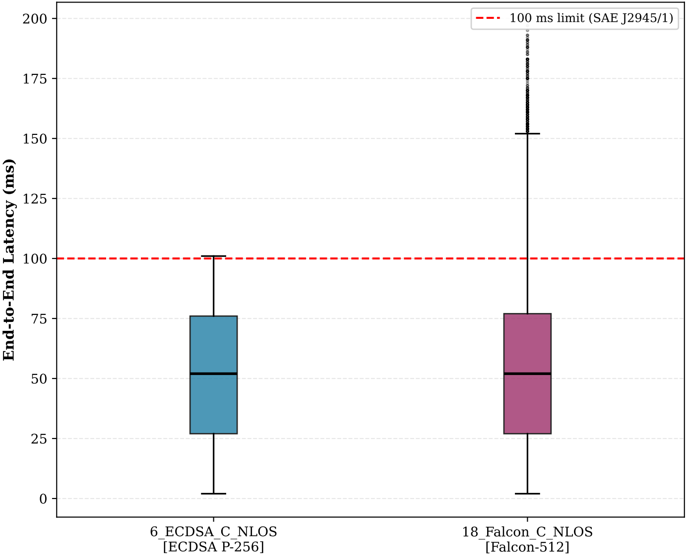
Latency Comparison — Scenario 6 vs Scenario 18
