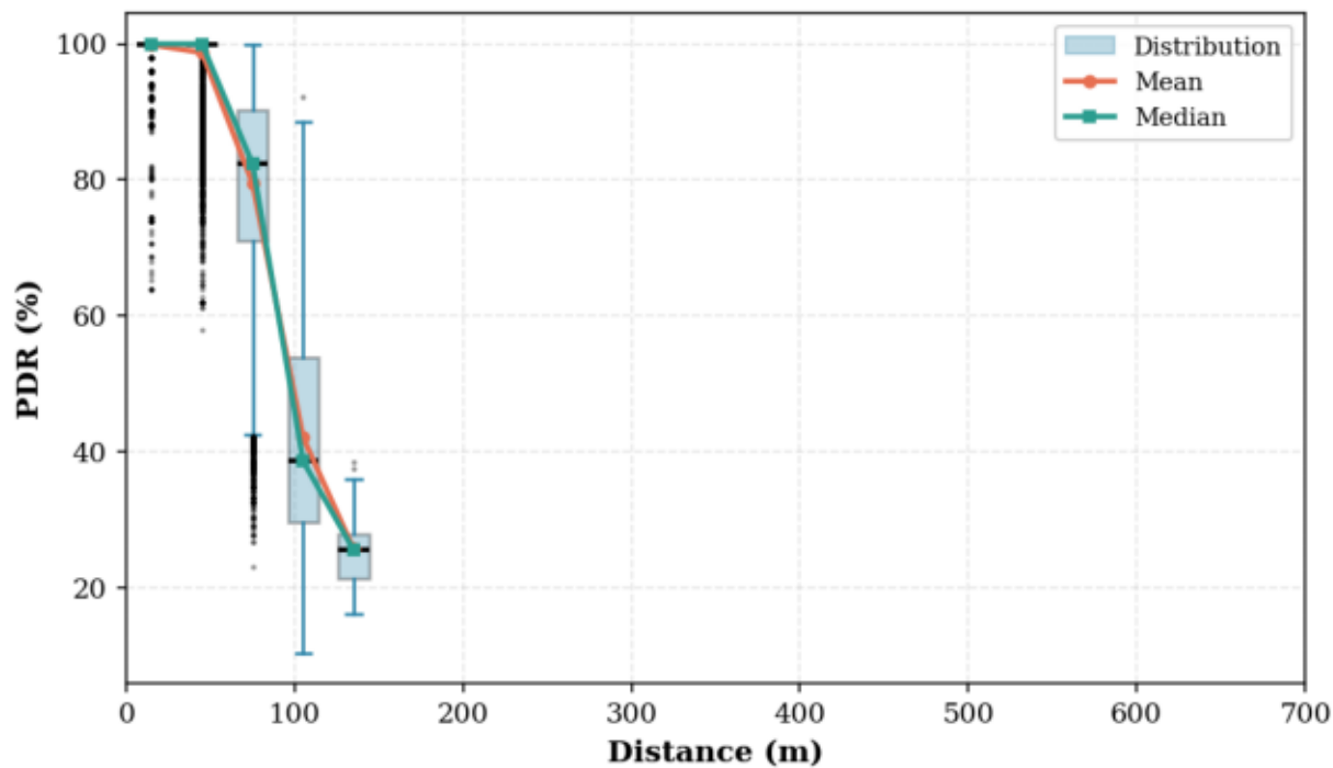
4_ECDSA_B_NLOS [ECDSA P-256]
