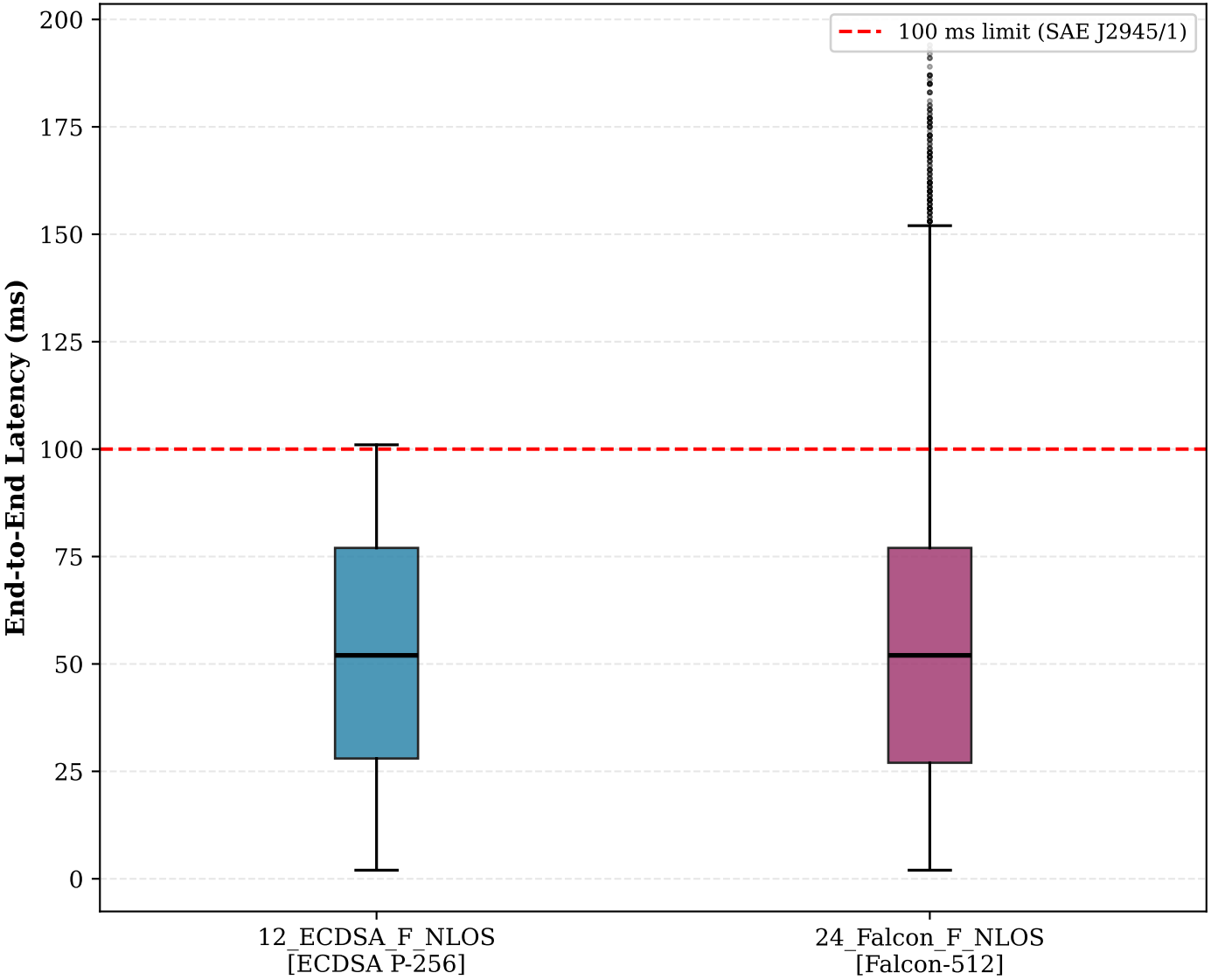
Latency Comparison — Scenario 12 vs Scenario 24
