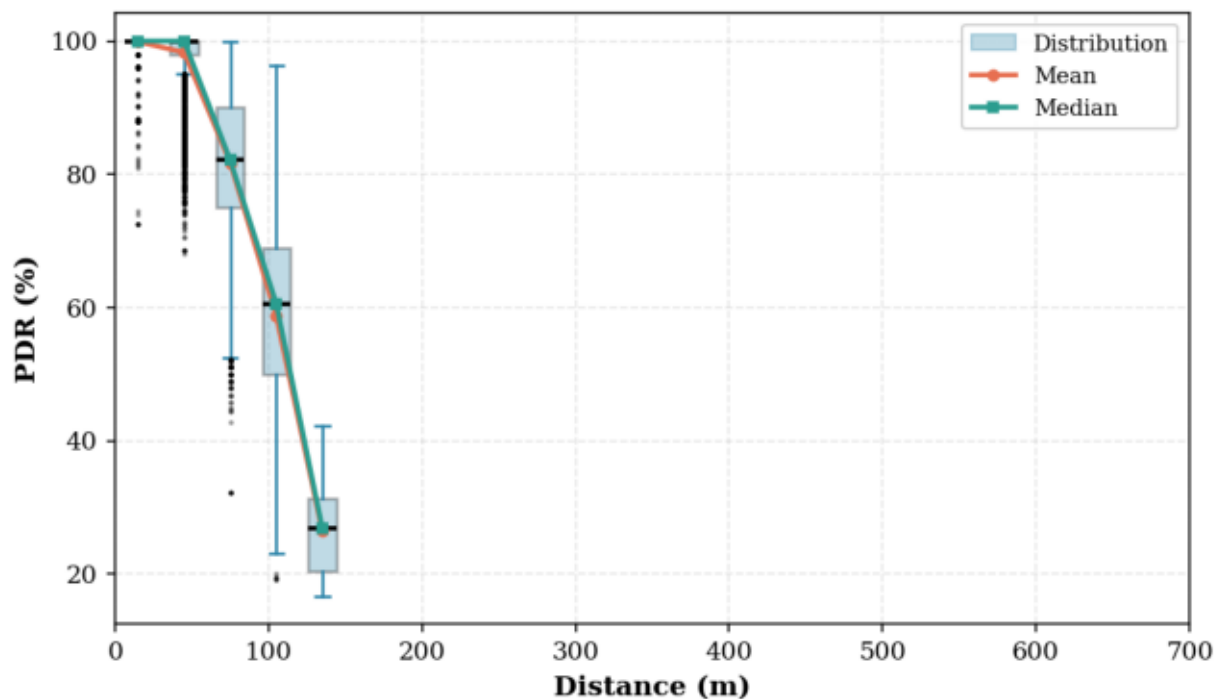
2_ECDSA_A_NLOS [ECDSA P-256]
