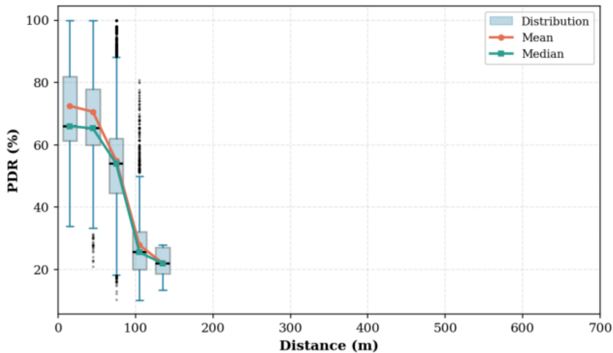
12_ECDSA_F_NLOS [ECDSA P-256]
