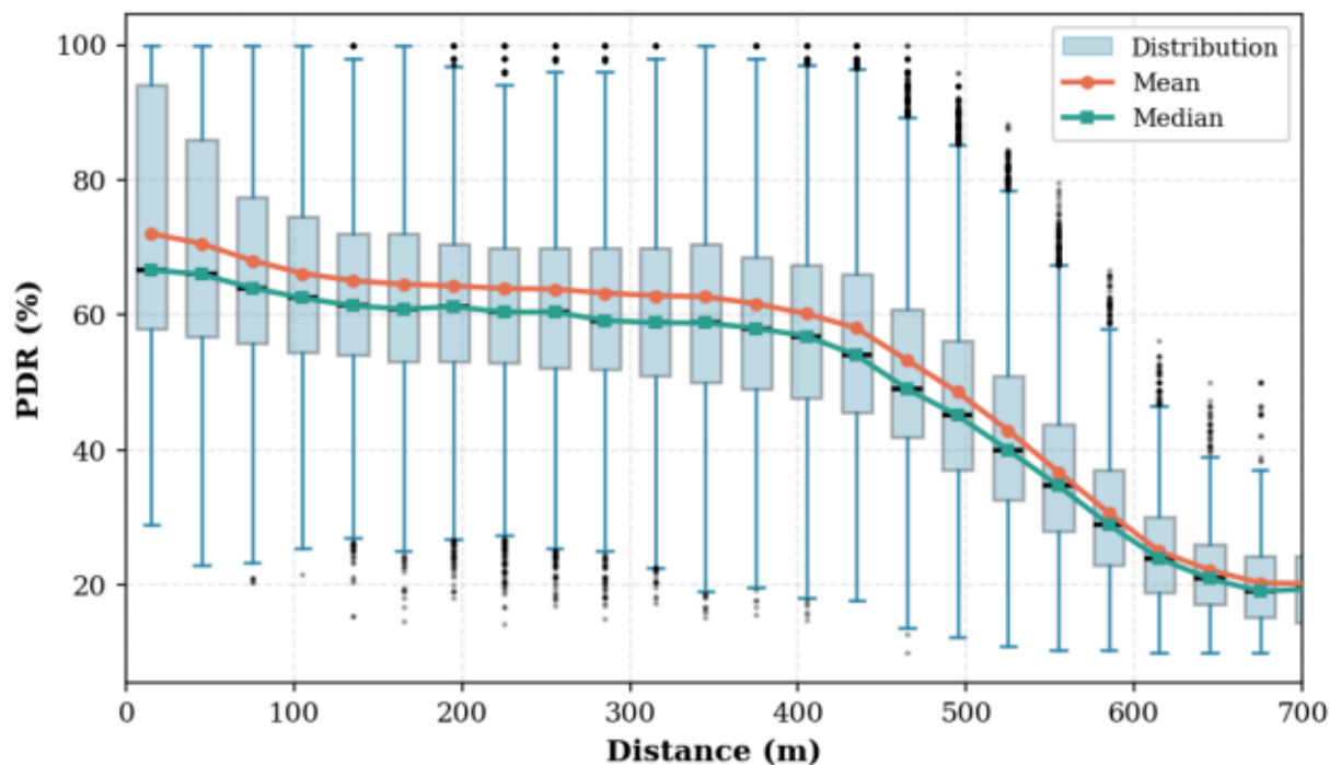
11_ECDSA_F_LOS [ECDSA P-256]
