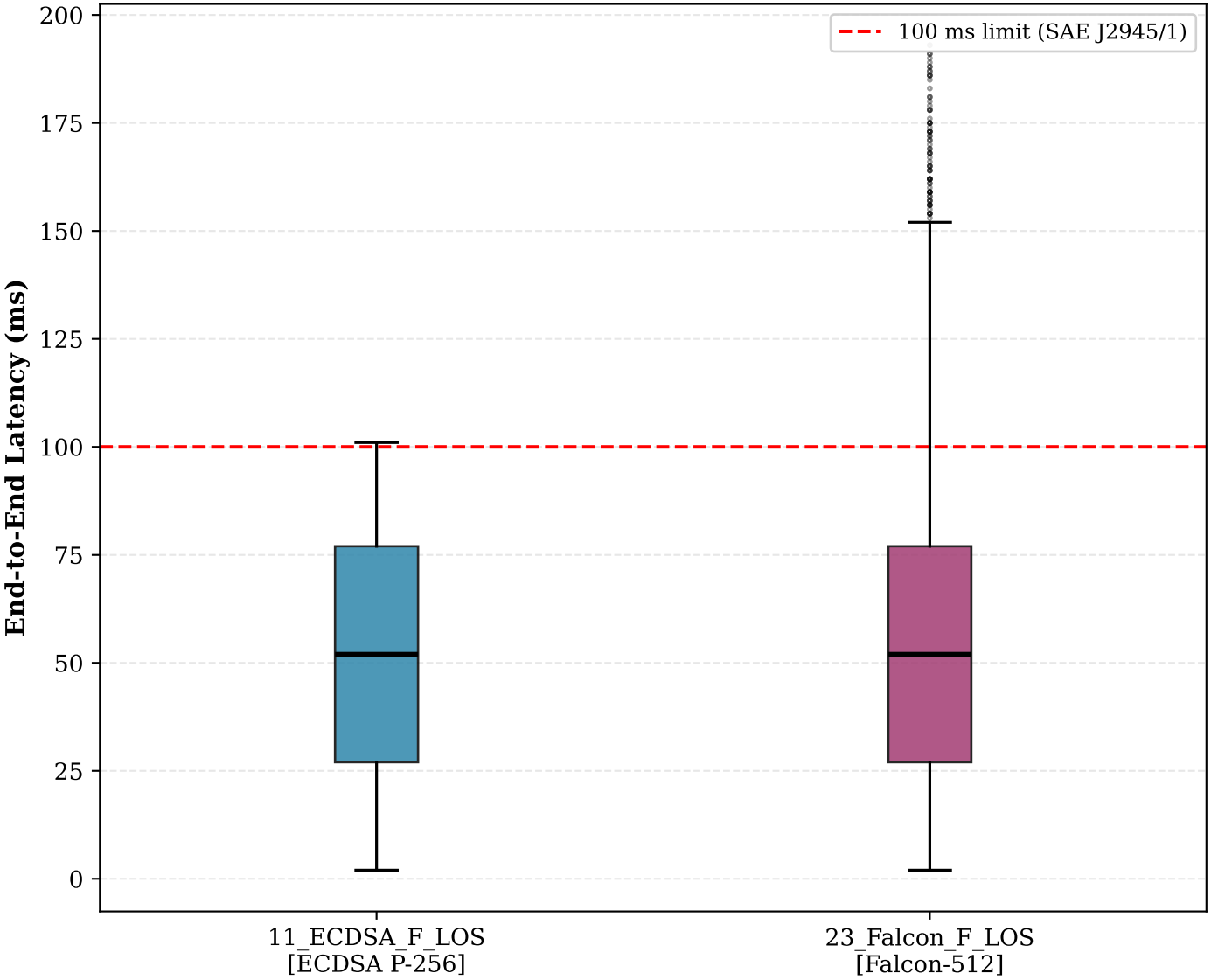
Latency Comparison — Scenario 11 vs Scenario 23
