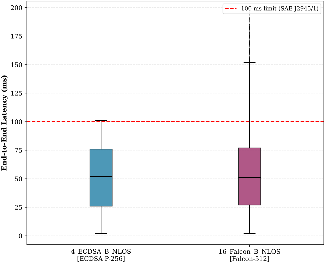
Latency Comparison — Scenario 4 vs Scenario 16
