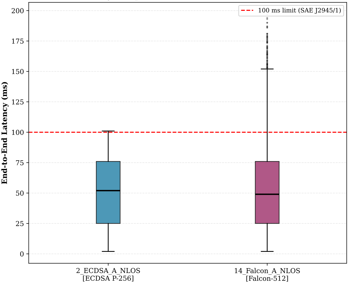
Latency Comparison — Scenario 2 vs Scenario 14
