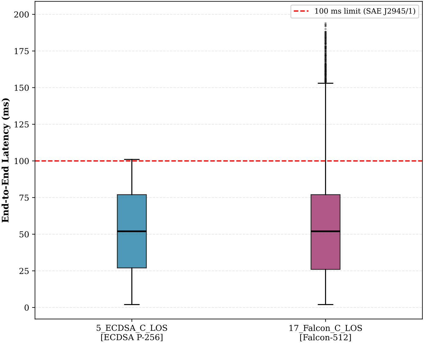
Latency Comparison — Scenario 5 vs Scenario 17
