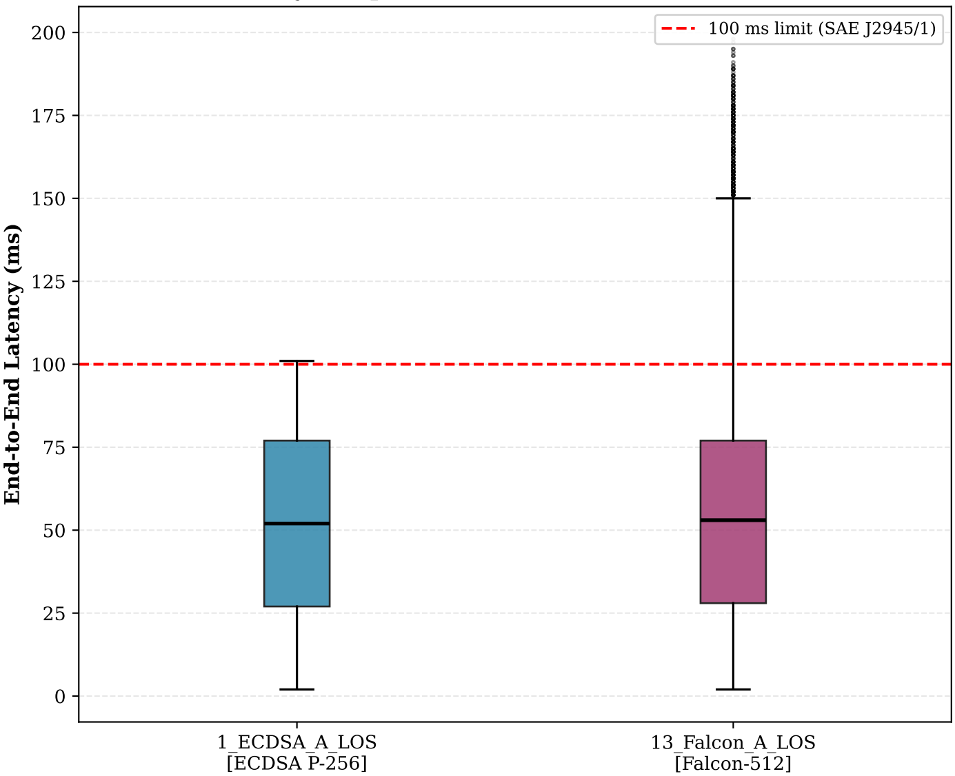
Latency Comparison — Scenario 1 vs Scenario 13
